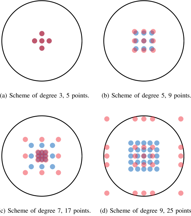
Fig. 1. Placement of sigma-points for Student's t, \vartheta = 9 , (red), Gaussian (blue) and a circle of radius 10 (black). (a) Sigma-point method of degree 3, (b) sigma-point method of degree 5, (c) sigma-point method of degree 7, and (d) sigma point method of degree 9. It is clear that Student's sigma-point method prefers to place the points further from origin.
