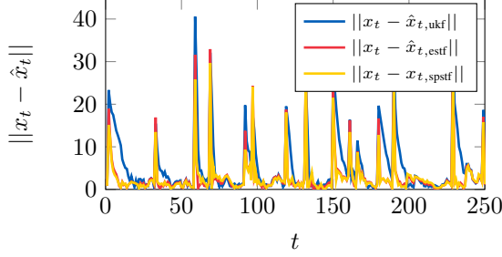
(b) The instantaneous norm of the error in state estimates, the degrees of freedom in Student's t filters were set to \vartheta = 4 .
